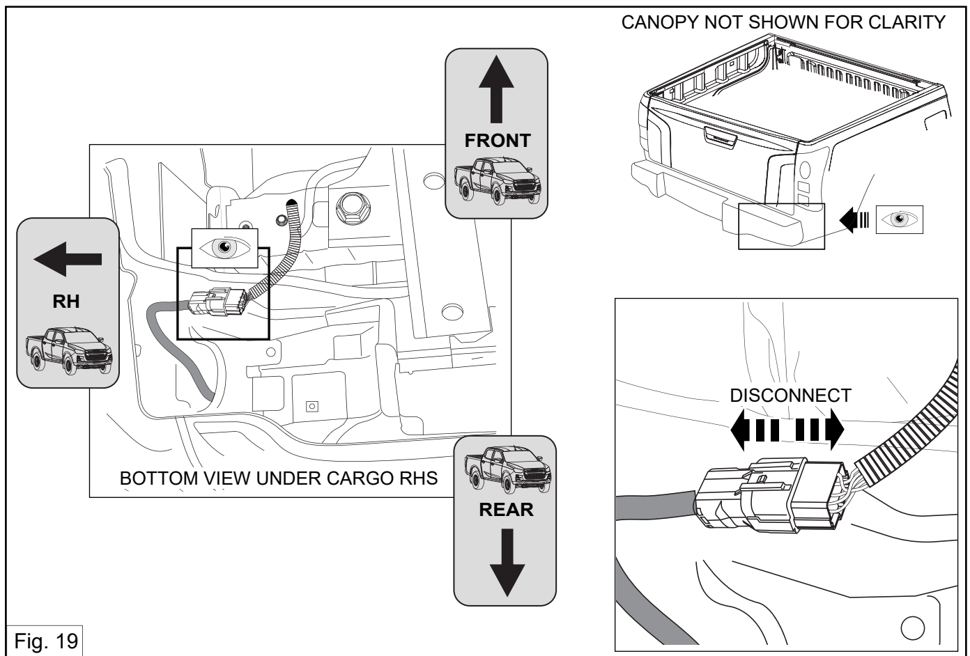
19. Locate and disconnect the RR Comb Lamp connector underneath the vehicle as shown.
