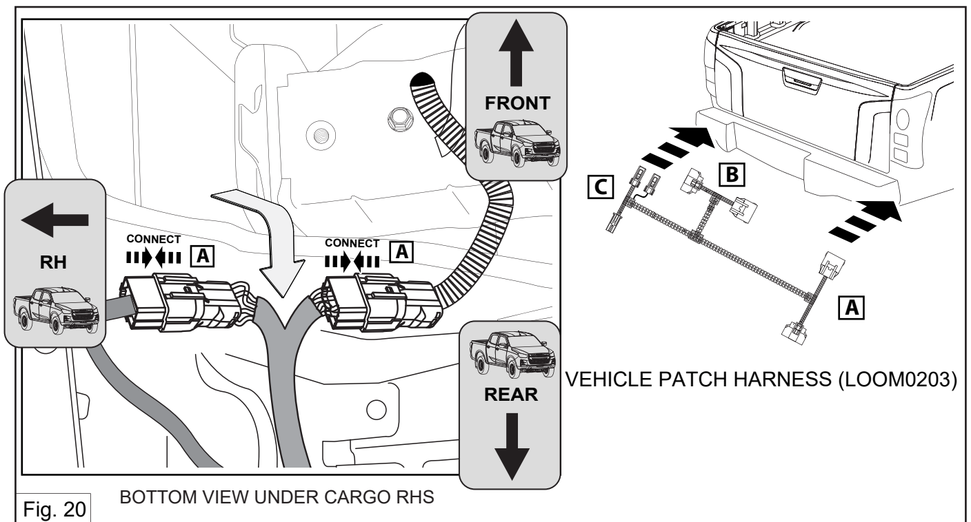
20. Bridge the male and female connectors from the RR Comb Lamp with the vehicle harness A connectors as shown vehicle patch harness (LOOM0203).
