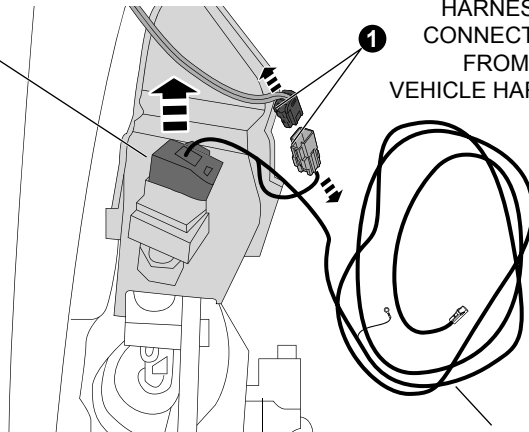
Diagram: 23 - DISCONNECT LAMP HARNESS
