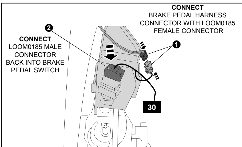
Diagram: 27 - CONNECT LOOM0185 TO THE BRAKE
