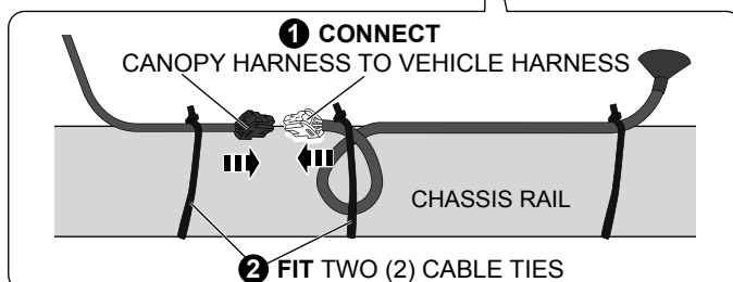
Diagram: 30 - CONNECT VEHICLE & CANOPY HARNESSES
