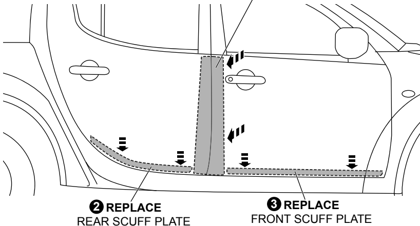
Diagram: 32 - REPLACE VEHICLE PARTS
