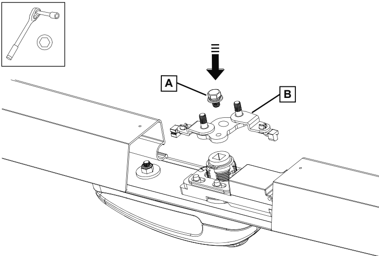
Diagram: 17 - REFIT CAM PLATE
