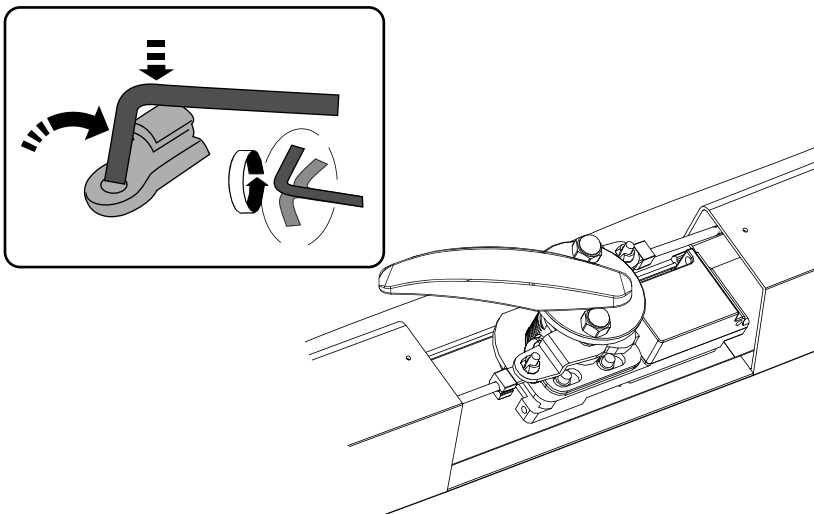
Diagram: 20 - LATCH ADJUSTMENT
