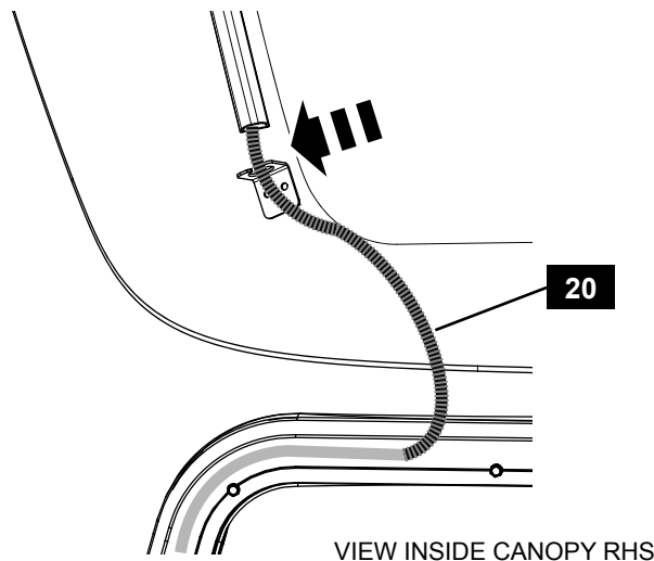
Diagram: 11 - SECURE WIRING
