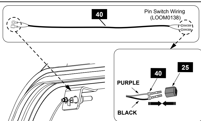
Diagram: 4 - CONNECT THE BRAKE LIGHT CONNECTOR
