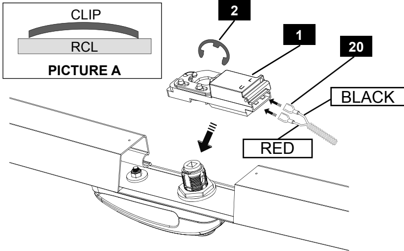
Diagram: 16 - FIT RCL
