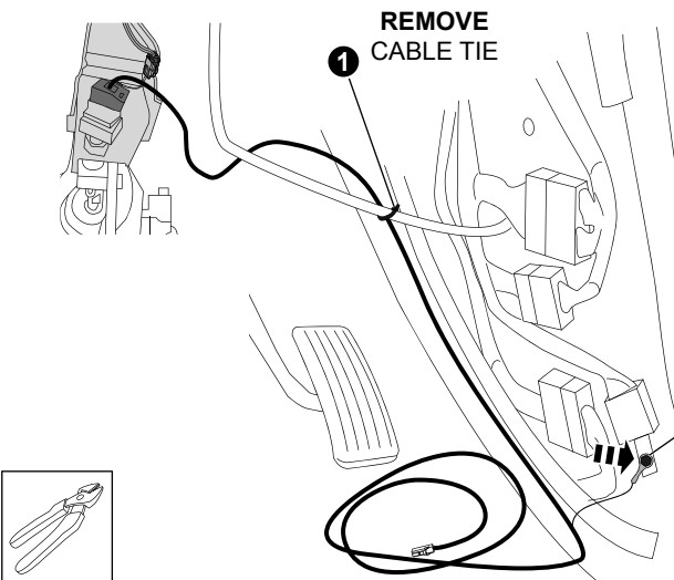
Diagram: 24 - CONNECT VEHICLE HARNESS
