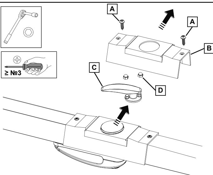
Diagram: 9 - REMOVE LOCK COVER
