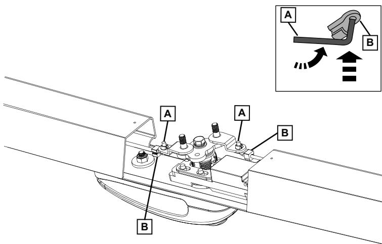
Diagram: 18 - CONNECT PULL RODS
