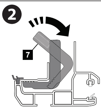
2 INSTALL 6 CLAMP TOPS INTO RAILS & SECURE WITH CLOTH TAPE
