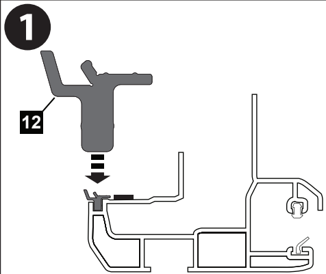
1 INSTALL RUBBER SEAL IN SIDE RAILS
